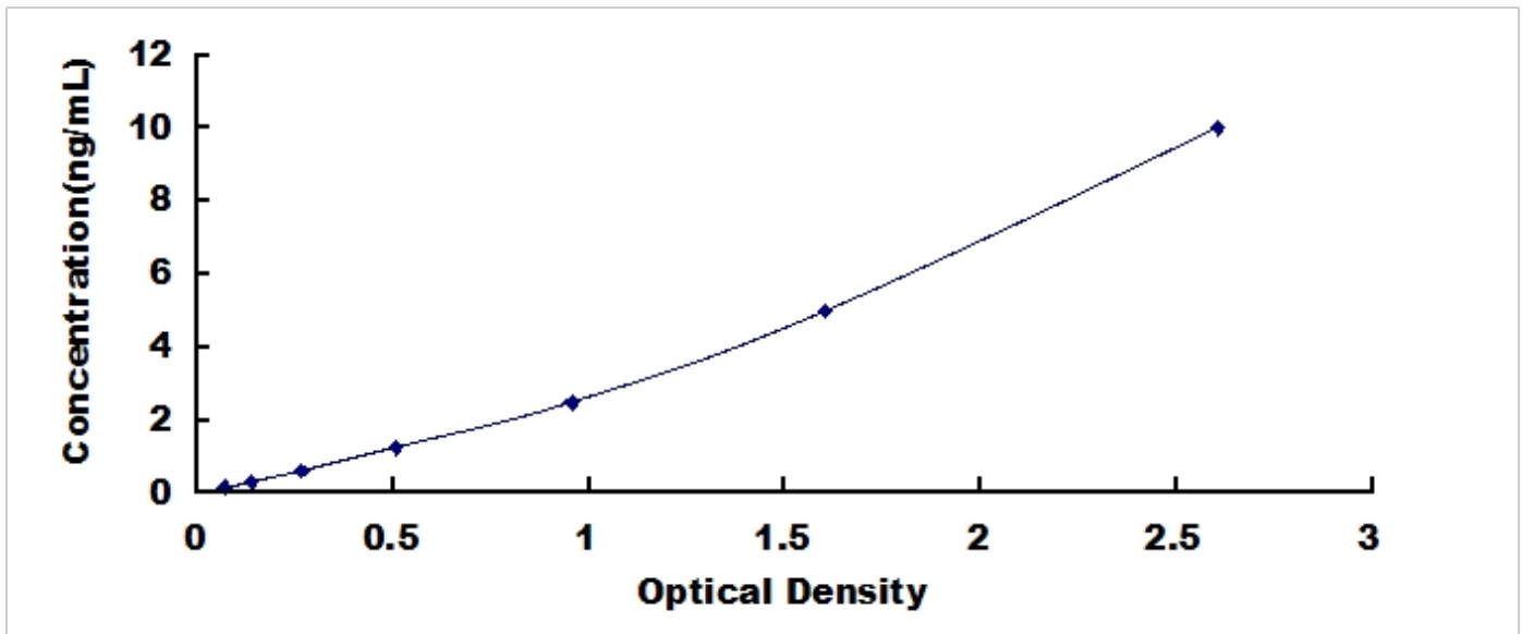
Typical Standard Curve for PRKACa, Human ELISA.
