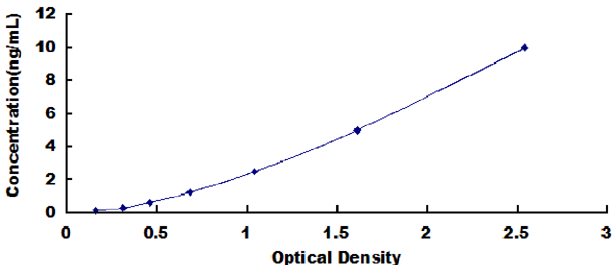
Typical Standard Curve for dLL3, Human ELISA.
