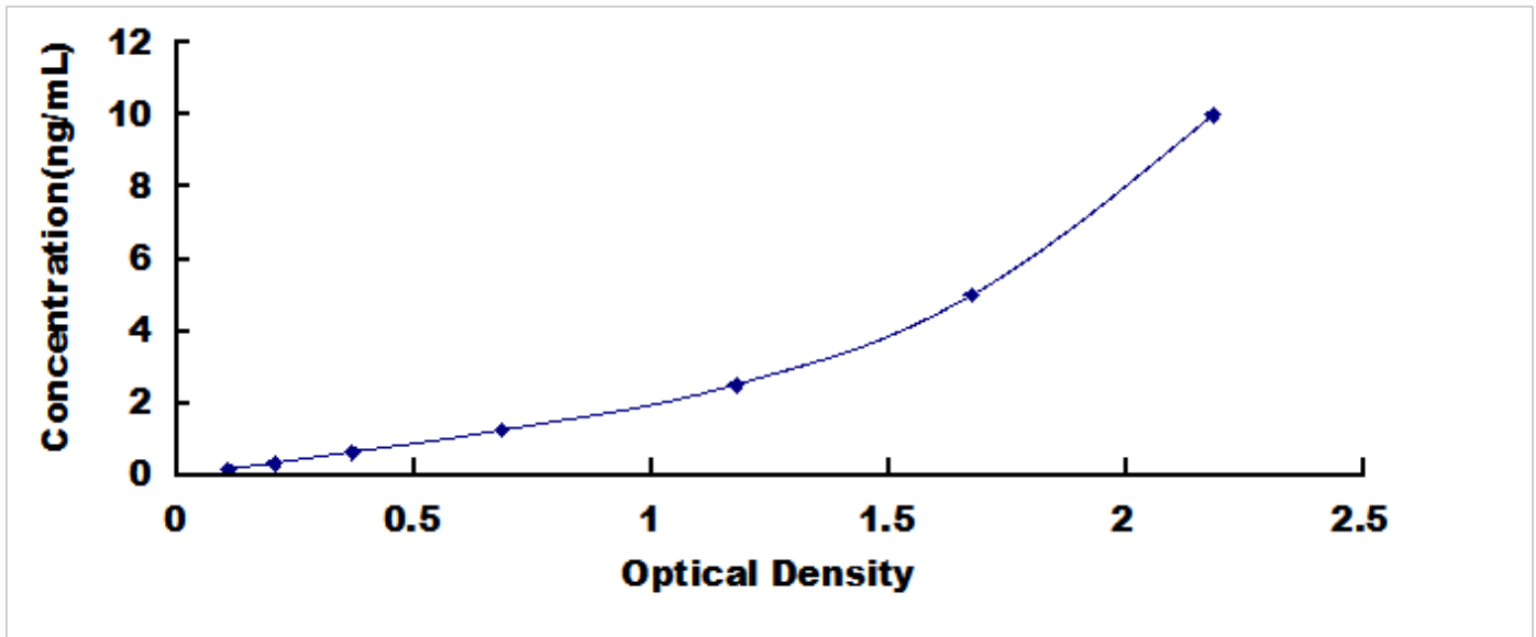
Typical Standard Curve for MDH1, Mouse ELISA.
