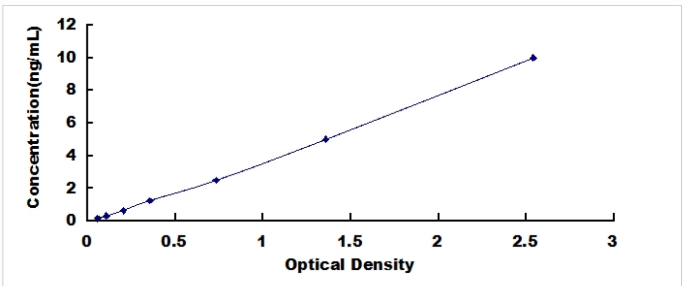
Typical Standard Curve for IDO, Rabbit ELISA.
