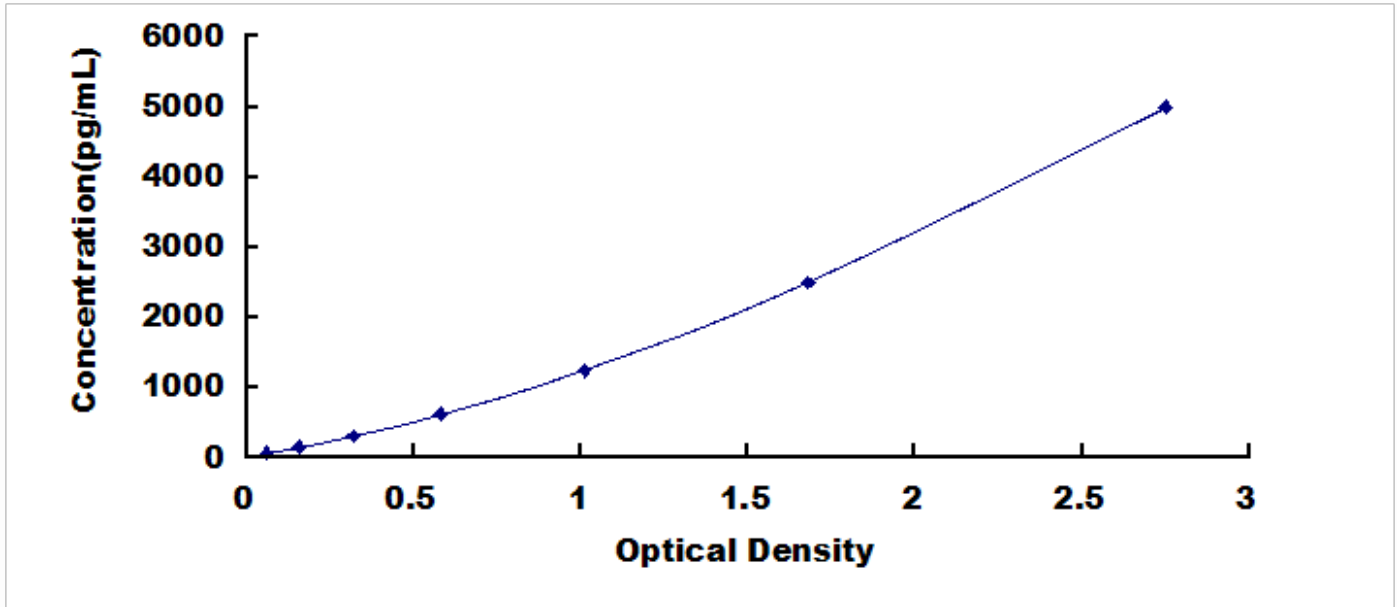
Typical Standard Curve for Ghrelin, rat ELISA.
