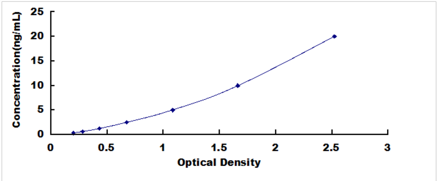
Typical Standard Curve for C3c, Mouse ELISA.
