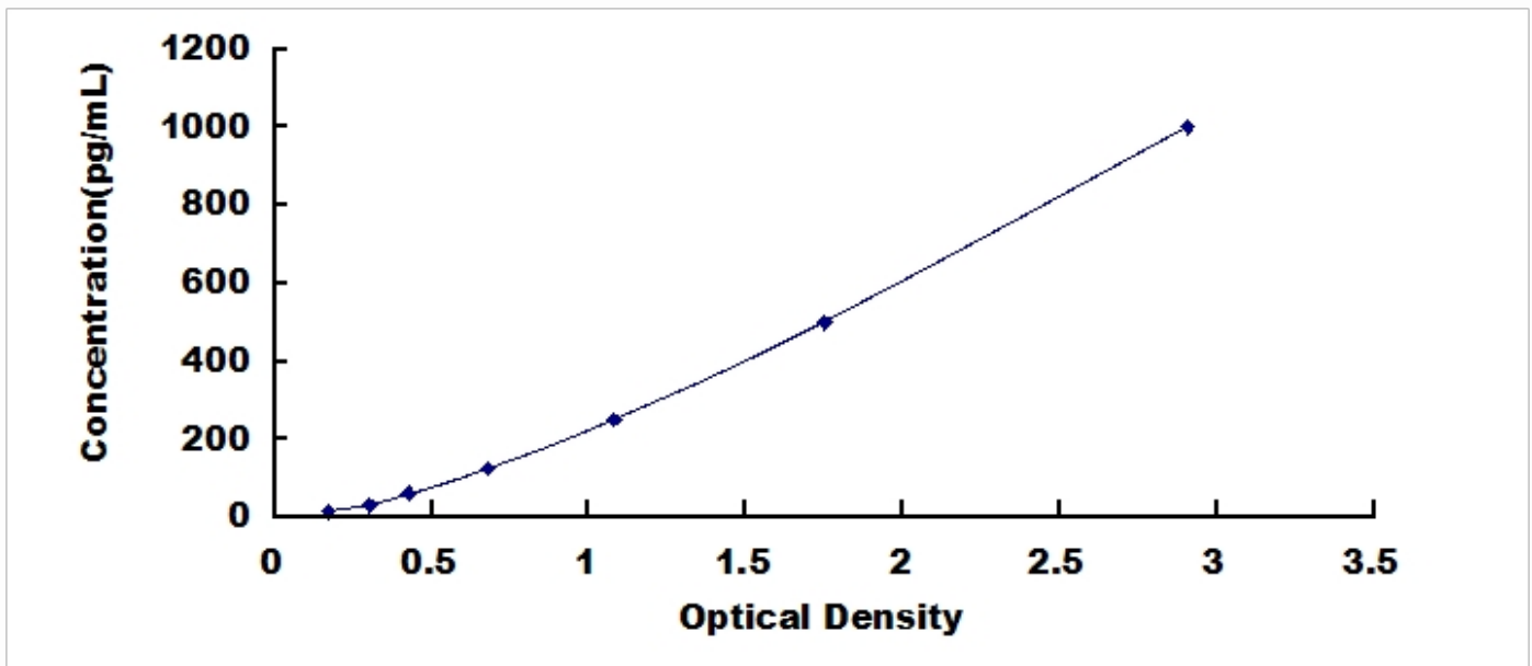
Typical Standard Curve for FABP2, Porcine ELISA.
