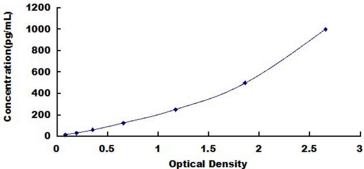
Typical Standard Curve for BNP, Rat ELISA.
