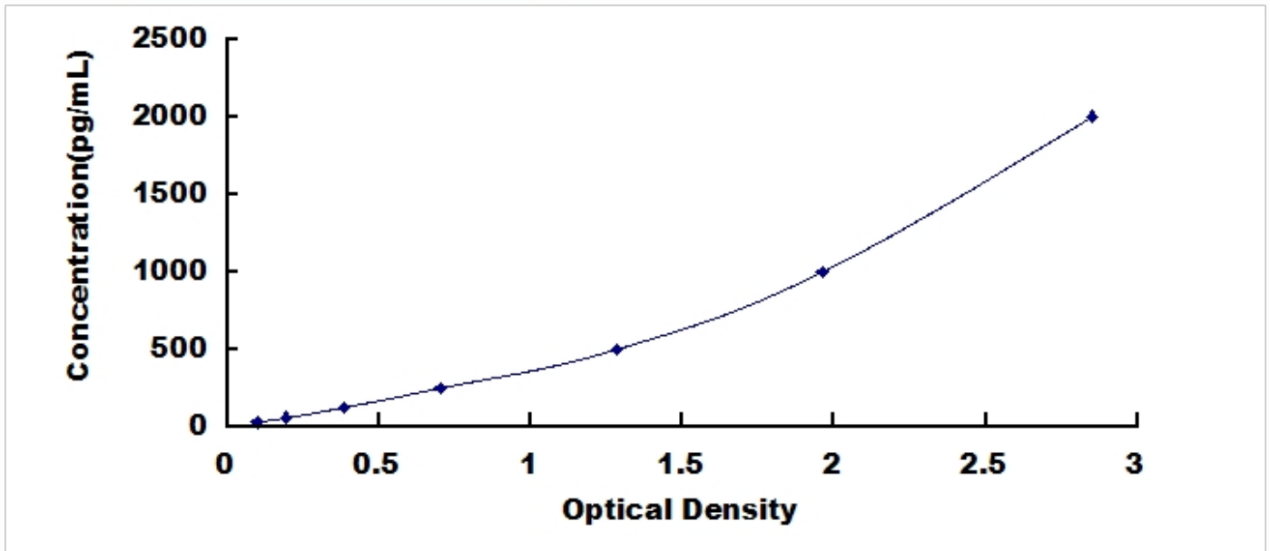
Typical Standard Curve for ADH2, Human ELISA.
