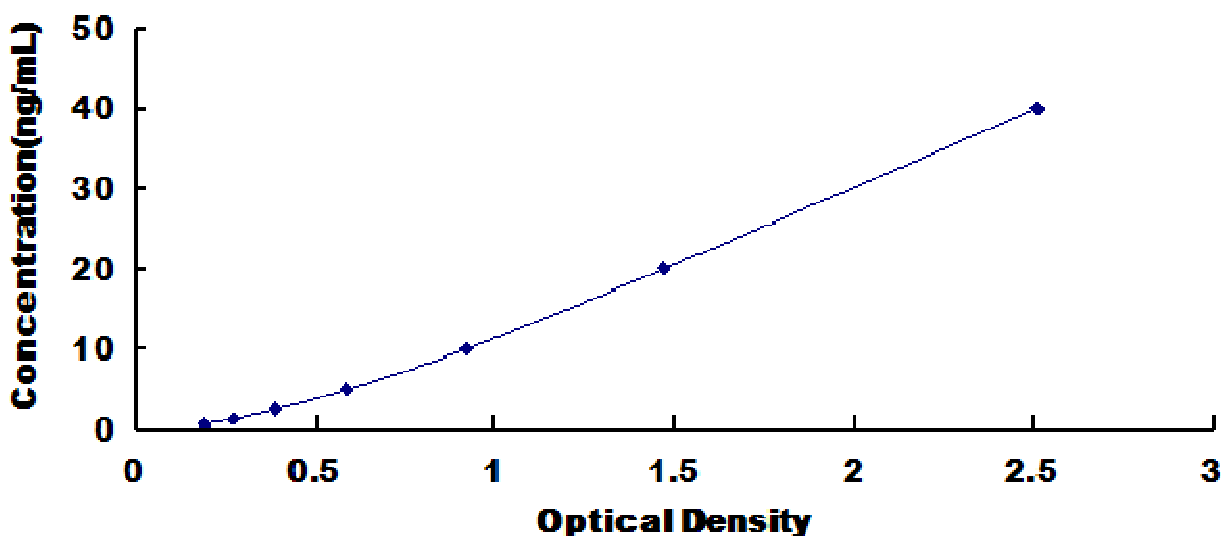
Typical Standard Curve for Rat ACTHR ELISA.
