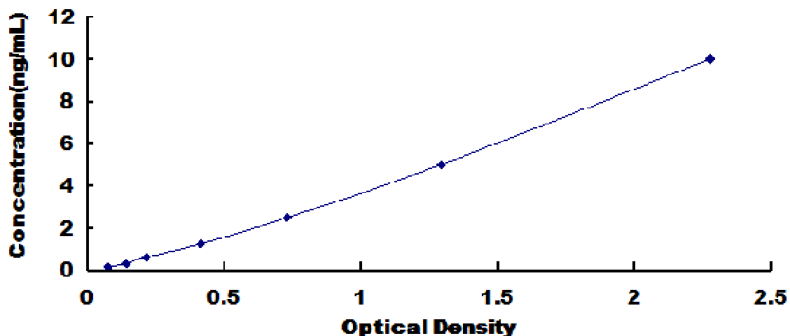
Typical Standard Curve for Human TWIST ELISA.
