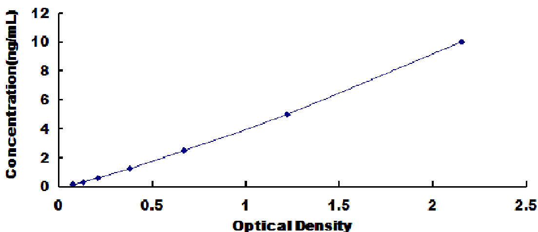
Typical Standard Curve for Human VNN1 ELISA.
