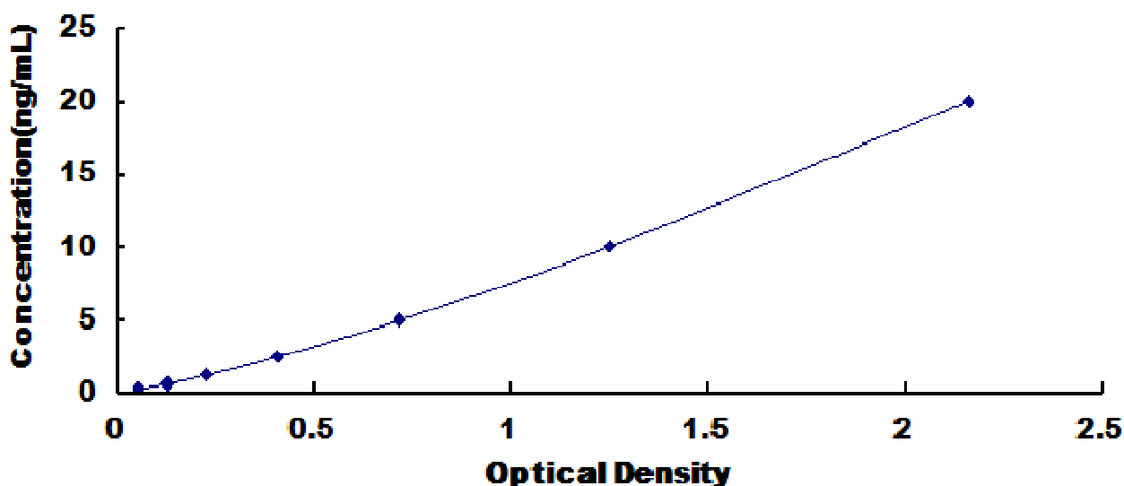
Typical Standard Curve for ADCY10, Mouse ELISA.
