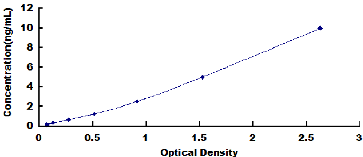
Typical Standard Curve for ACTg2, Human ELISA.
