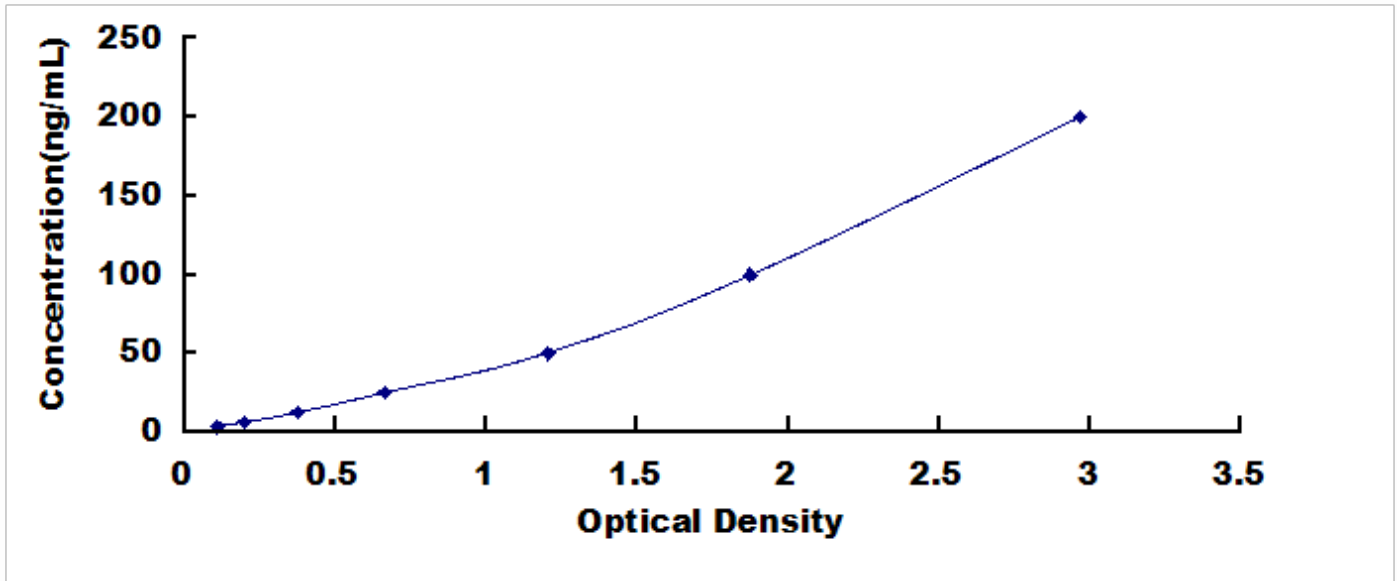
Typical Standard Curve for CLU, Canine ELISA.
