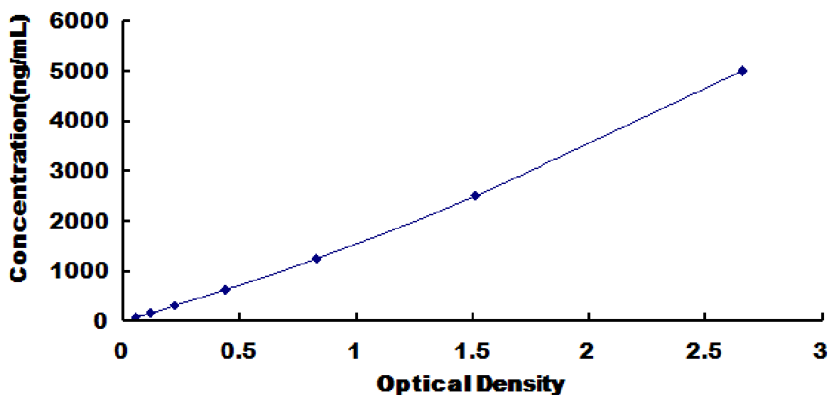
Typical Standard Curve for Porcine Hpt ELISA.
