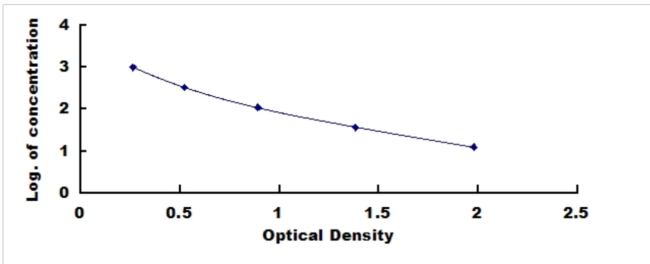
Typical Standard Curve for FGF2, Bovine ELISA.
