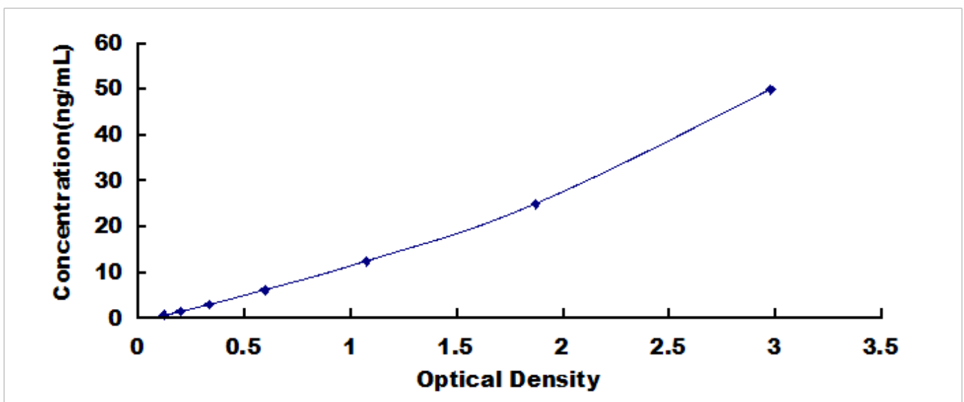
Typical Standard Curve for SOD3, Rabbit ELISA.
