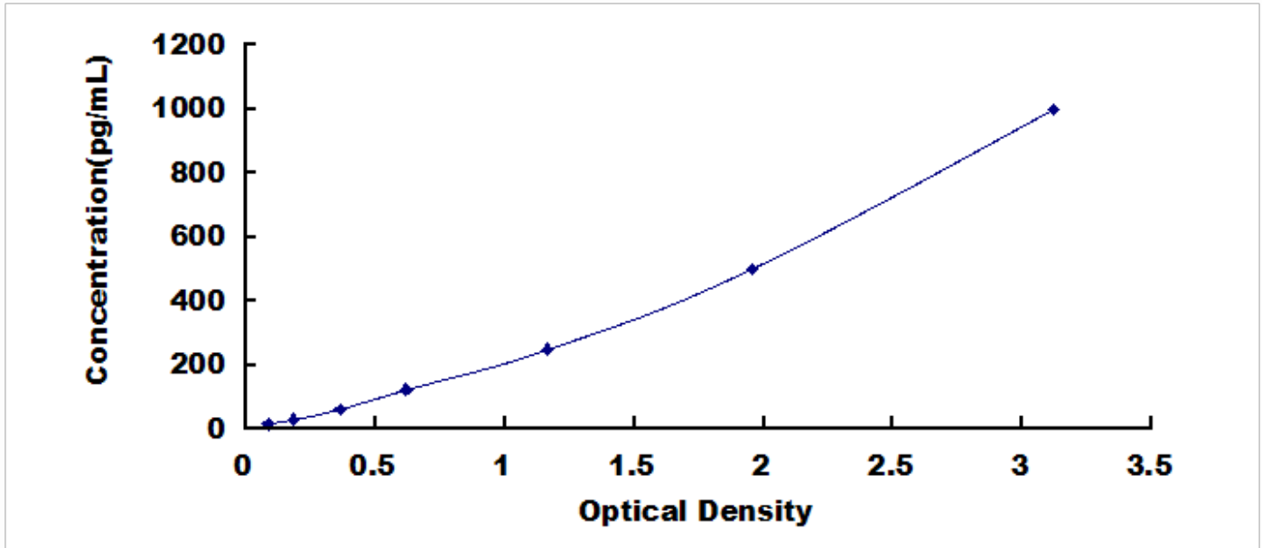
Typical Standard Curve for IL8, Rabbit ELISA.
