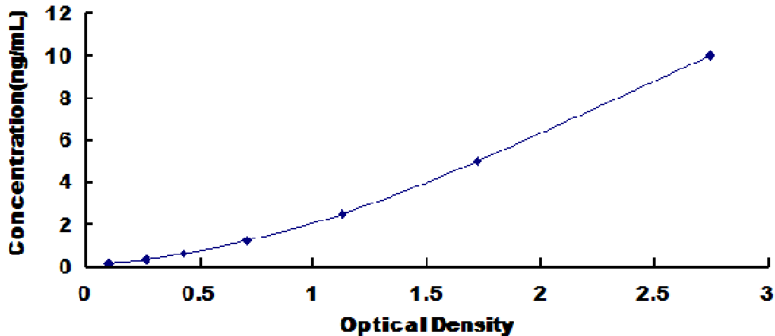
Typical Standard Curve for BDNF, Cavia ELISA.
