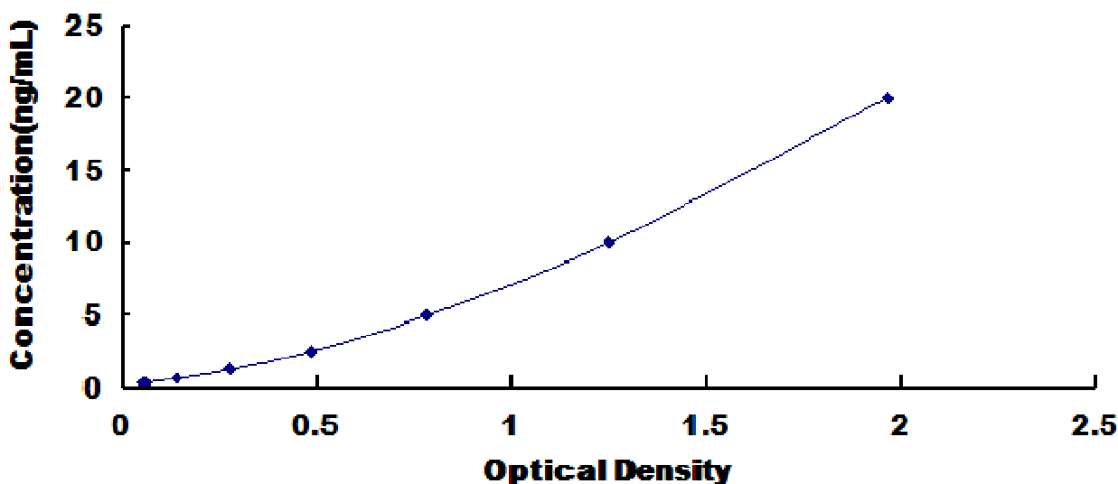
Typical Standard Curve for Human RBM24 ELISA.
