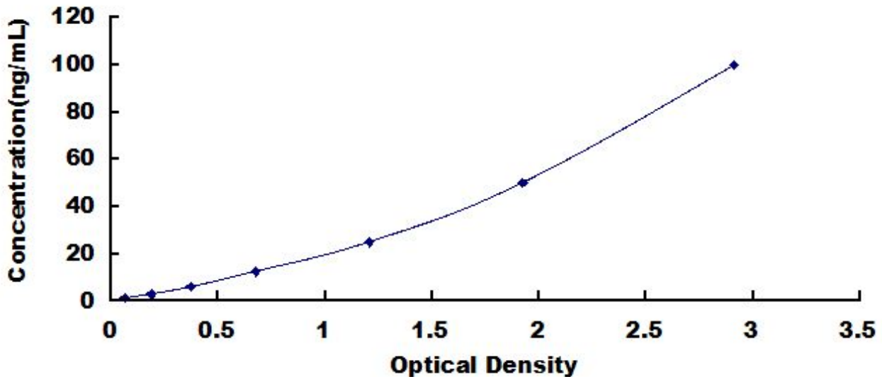
Typical Standard Curve for CTHRC1, Human ELISA.
