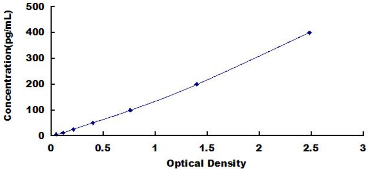
Typical Standard Curve for RETNLb, Mouse ELISA.
