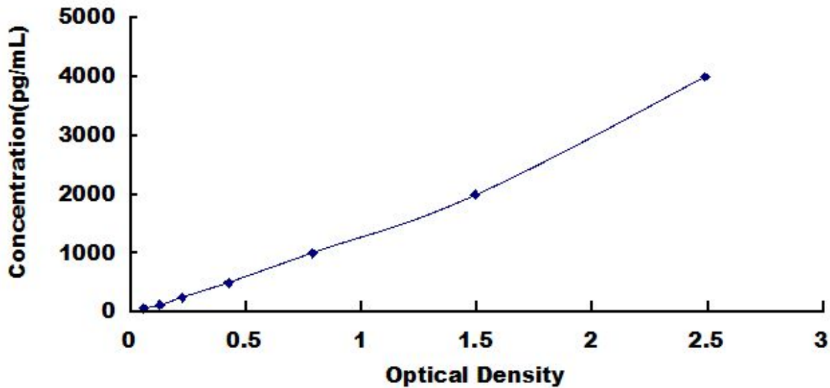
Typical Standard Curve for RETNLb, Human ELISA.
