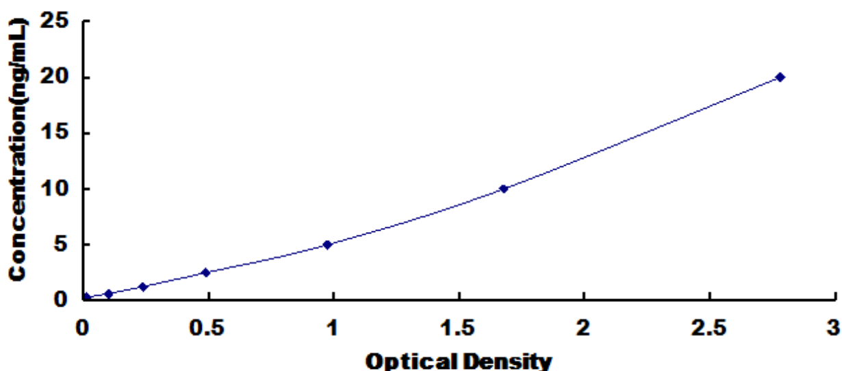
Typical Standard Curve for Human RCBTB2 ELISA.
