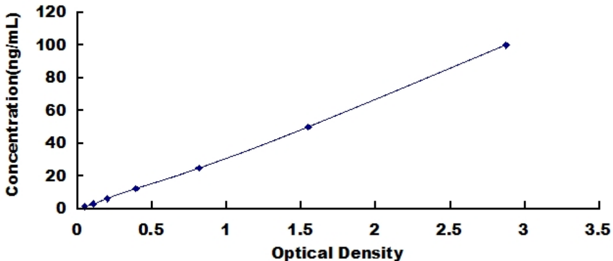
Typical Standard Curve for SEMA3A, Human ELISA.
