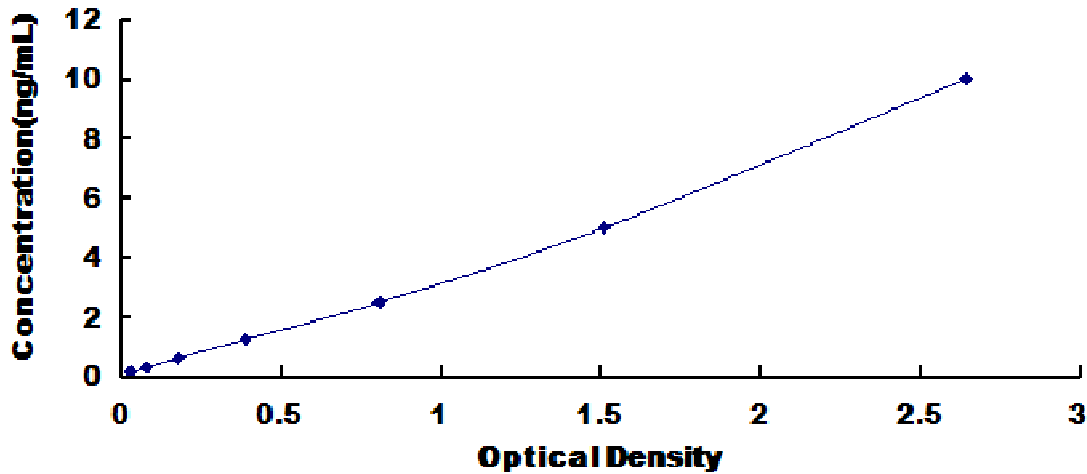
Typical Standard Curve for WNT3, Rat ELISA.
