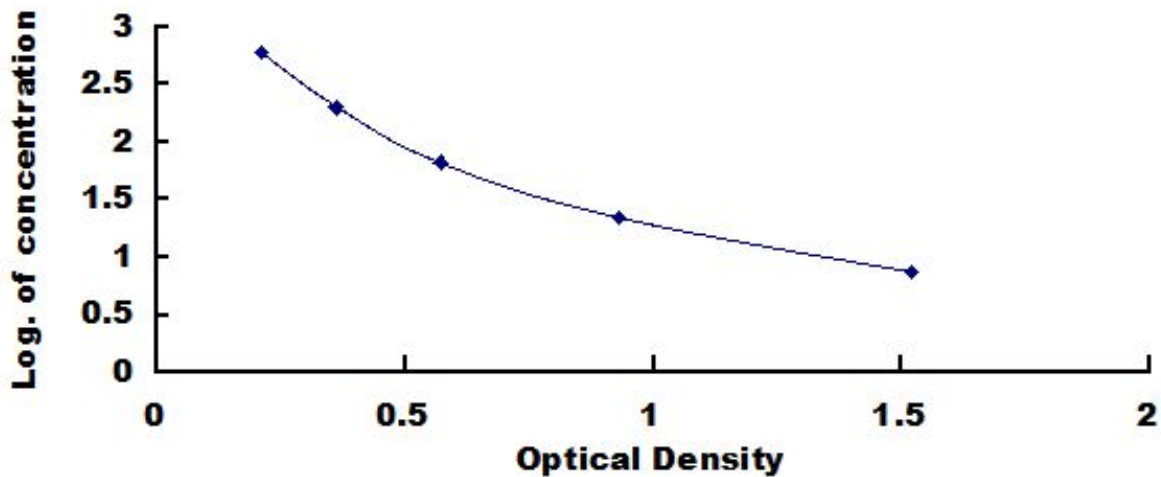
Typical Standard Curve for Lactic Acid ELISA.
