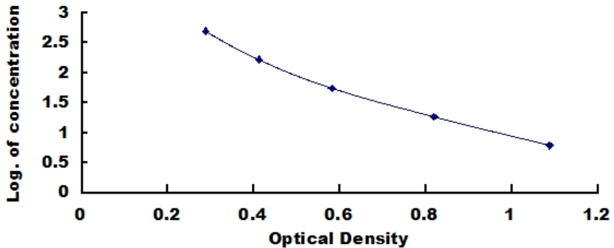
Typical Standard Curve for Hemoglobin, Ovine ELISA.
