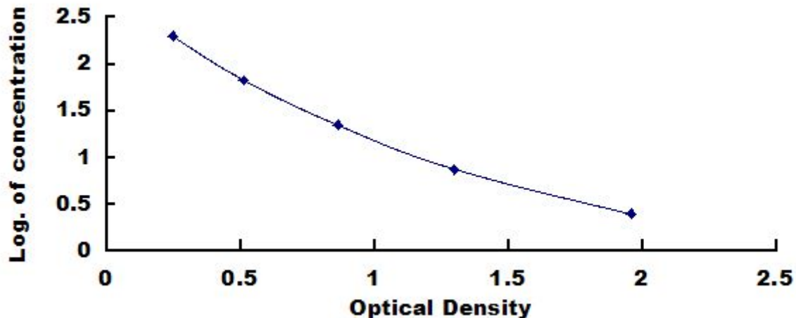
Typical Standard Curve for PIIICP, Human ELISA.
