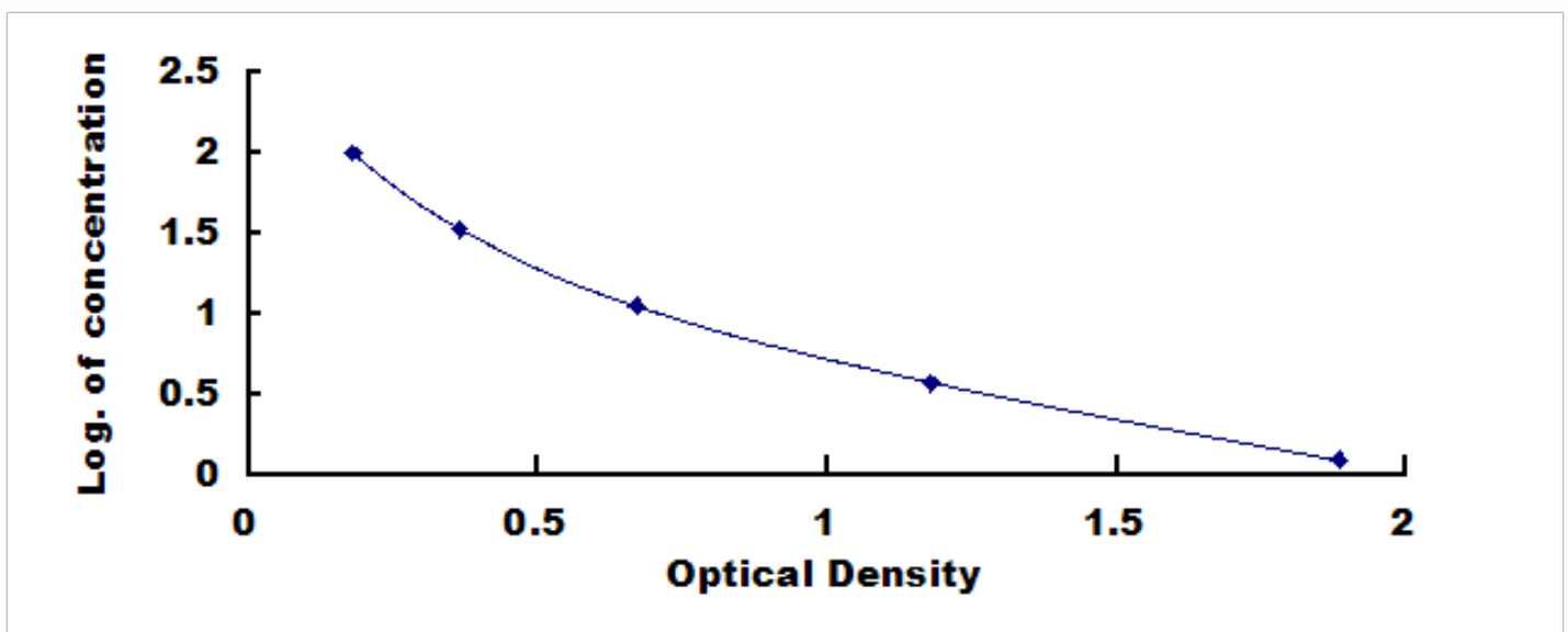
Typical Standard Curve for sIgA, Porcine ELISA.
