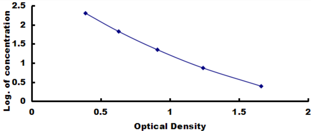
Typical Standard Curve for OxLDL, Rat ELISA.
