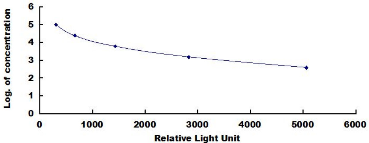
Typical Standard Curve for DHEA, CLIA.
