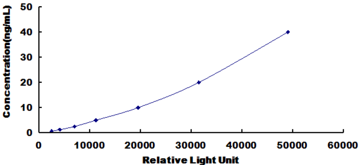
Typical Standard Curve for Rat BNIP3 CLIA.
