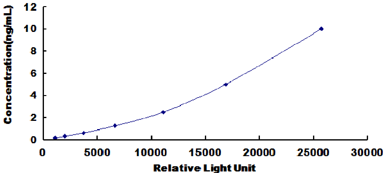
Typical Standard Curve for Human ZNRD1 CLIA.
