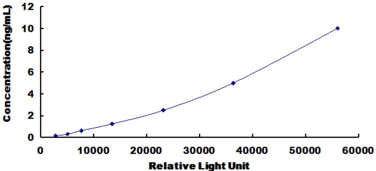
Typical Standard Curve for Human IDS CLIA.
