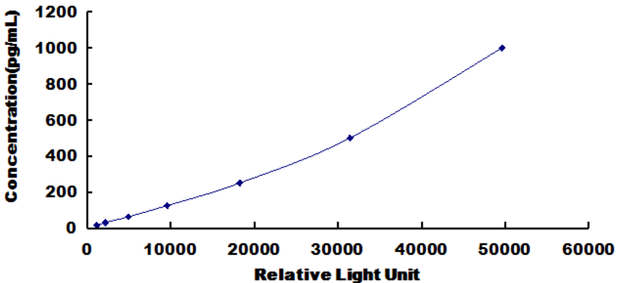
Typical Standard Curve for Mouse IFNa13 CLIA.
