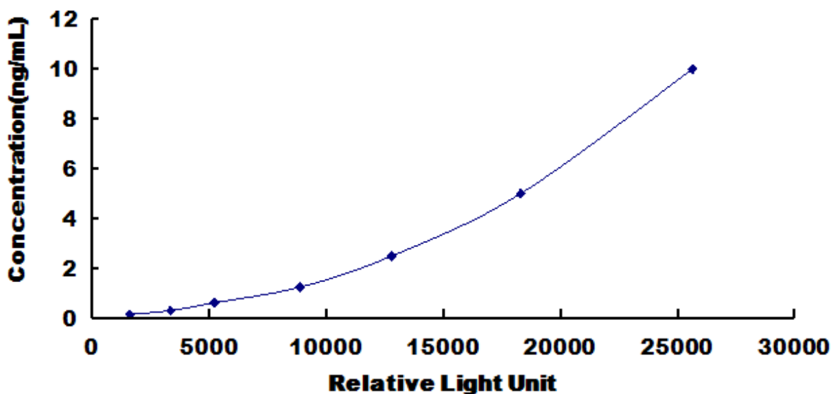
Typical Standard Curve for Rat BRAK CLIA.
