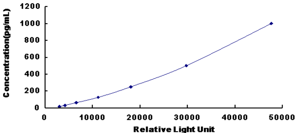
Typical Standard Curve for Human CCL14 CLIA.
