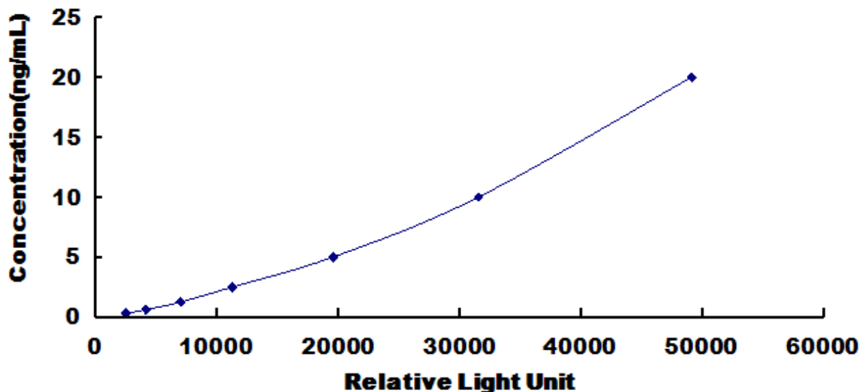
Typical Standard Curve for Human MUC5AC CLIA.
