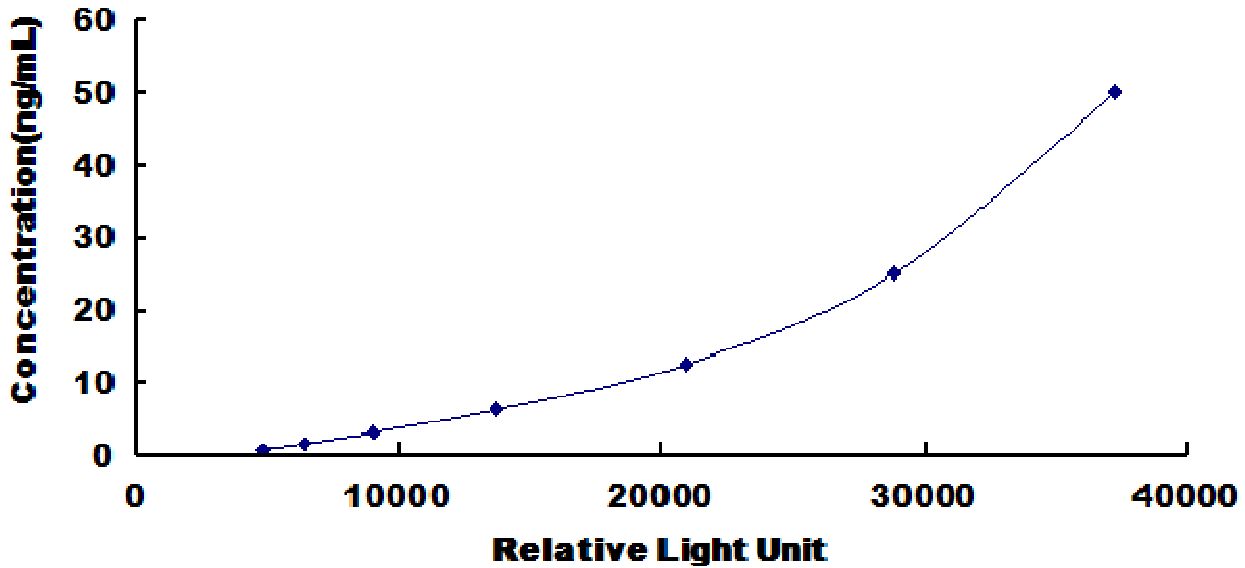
Typical Standard Curve for Bovine sIgA CLIA.
