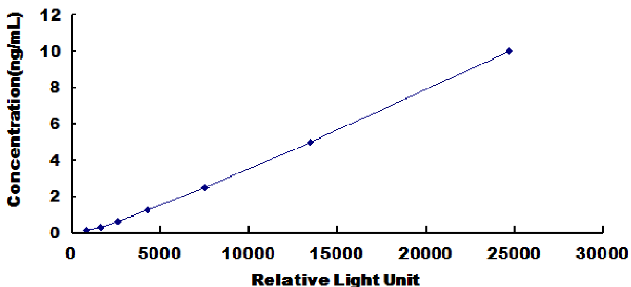
Typical Standard Curve for Human XPC CLIA.
