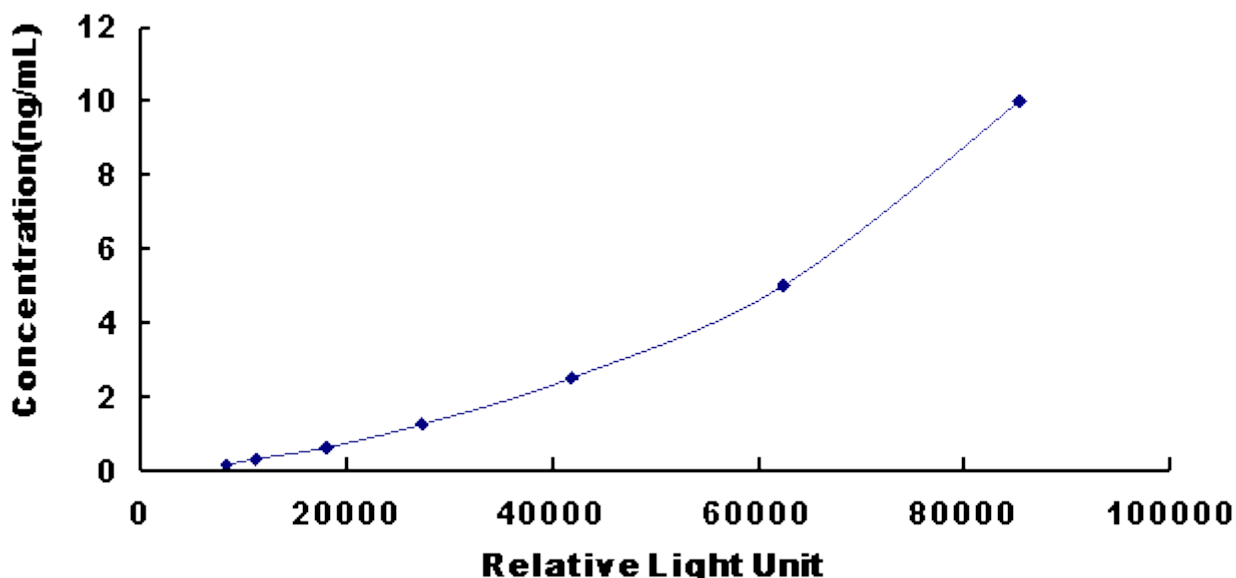
Typical Standard Curve for Porcine TIMP4 CLIA.
