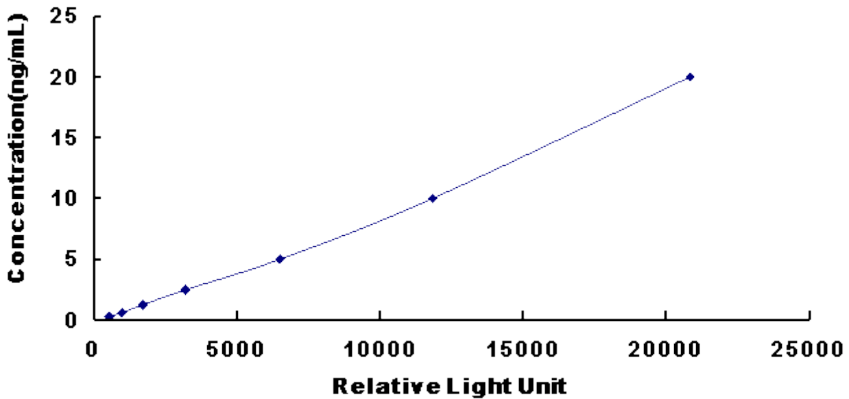
Typical Standard Curve for Gallus CCKAR CLIA.
