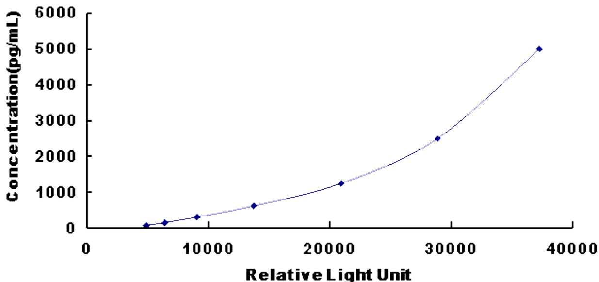
Typical Standard Curve for Human MMP3 CLIA.
