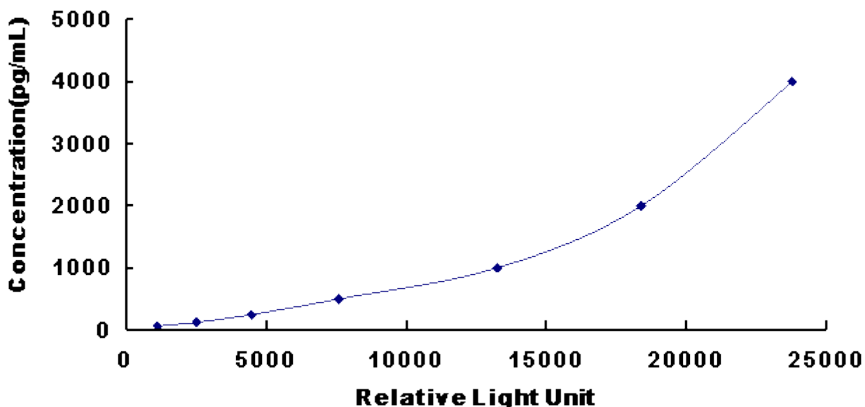
Typical Standard Curve for Equine MMP3 CLIA.
