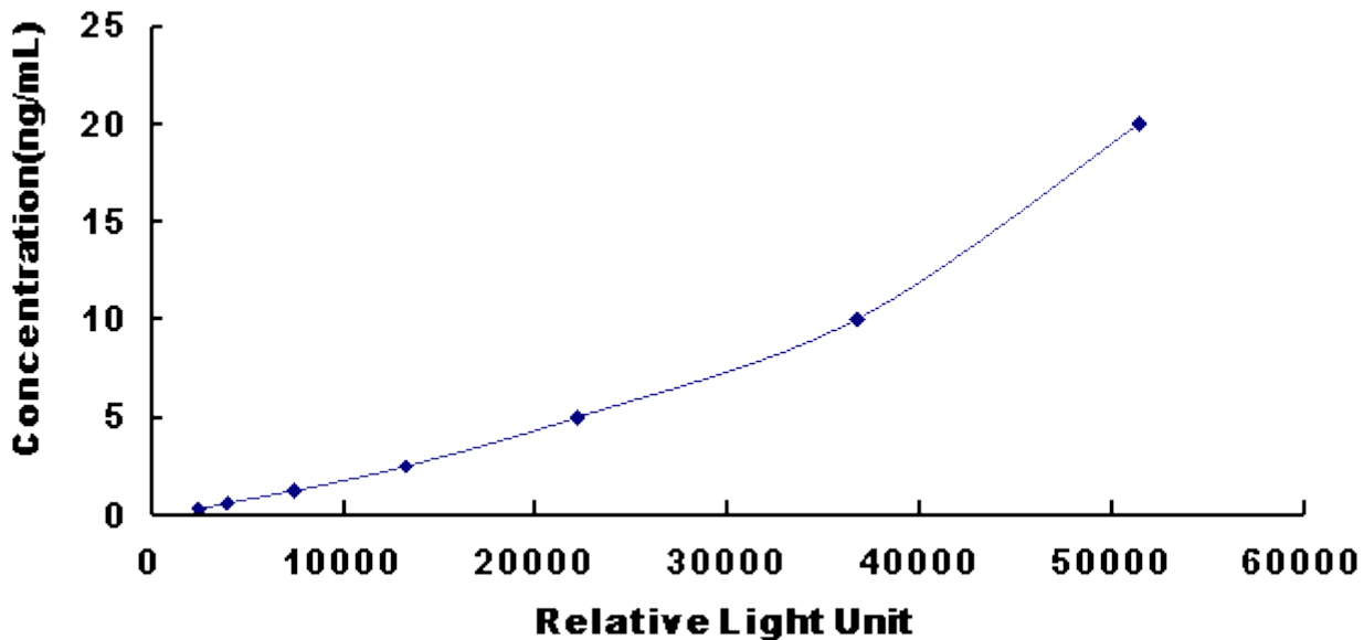
Typical Standard Curve for Canine MMP3 CLIA.
