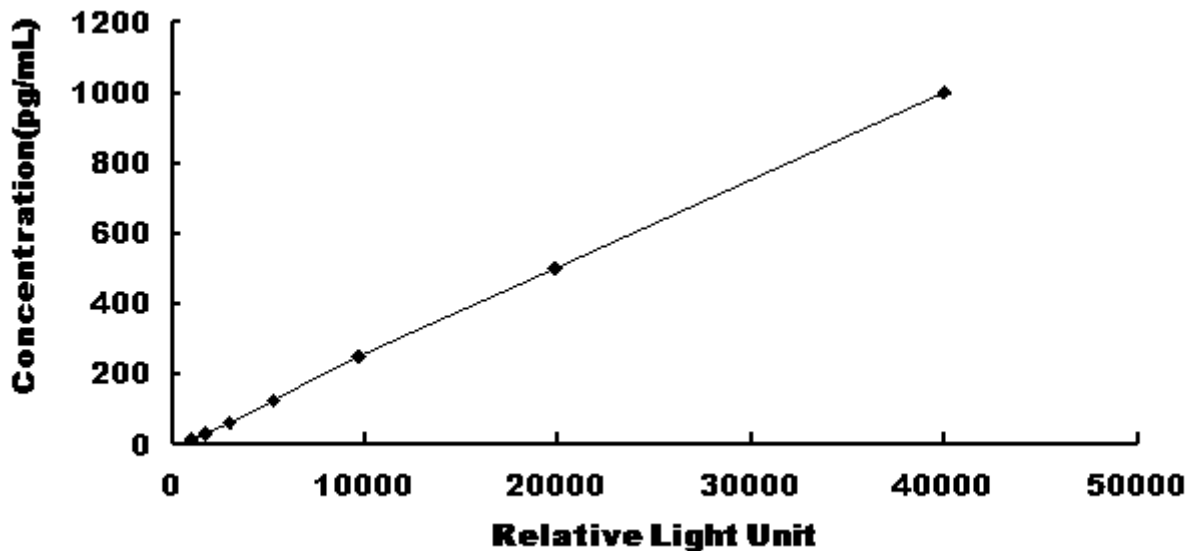
Typical Standard Curve for Simian IFNg CLIA.
