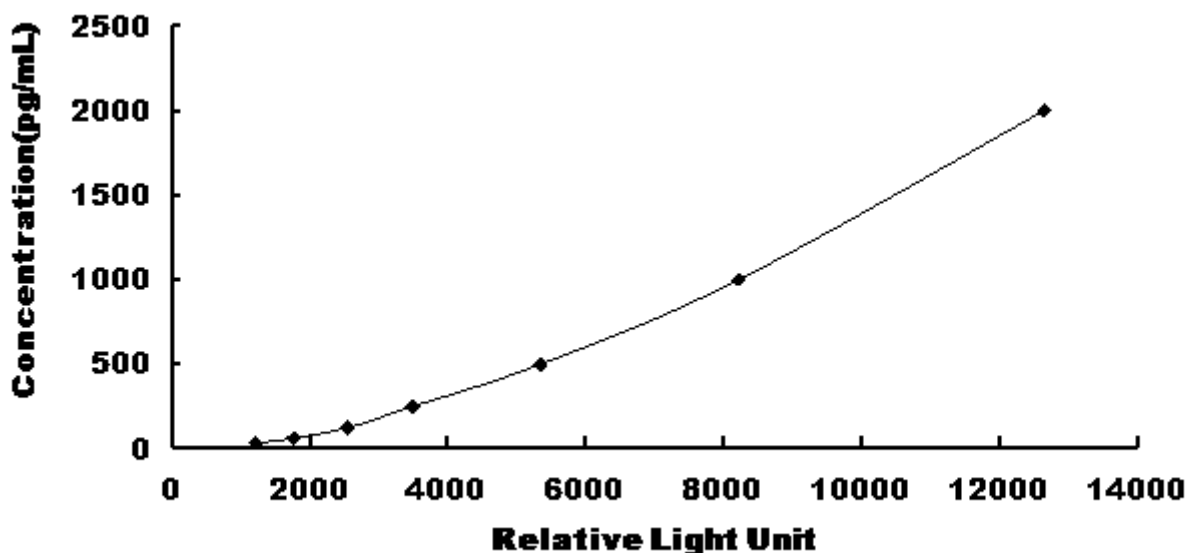
Typical Standard Curve for Mouse IFN \gamma CLIA.
