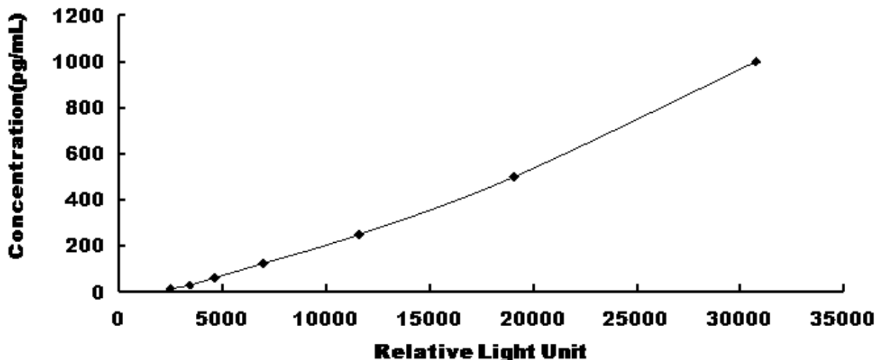
Typical Standard Curve for Mouse HGF CLIA.
